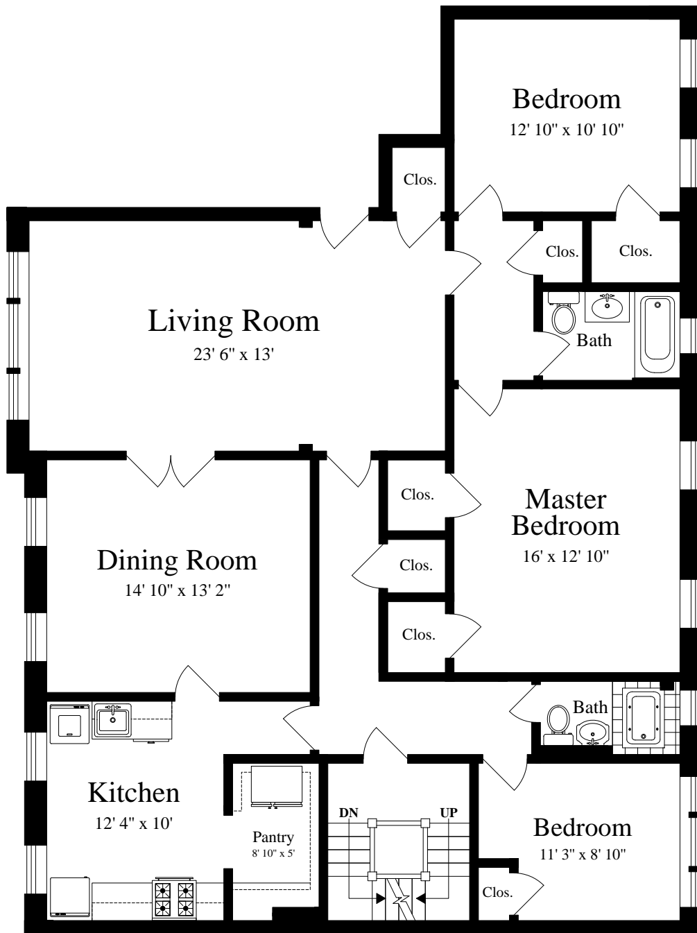
FIRST FLOOR (ceiling = 8' 6")
