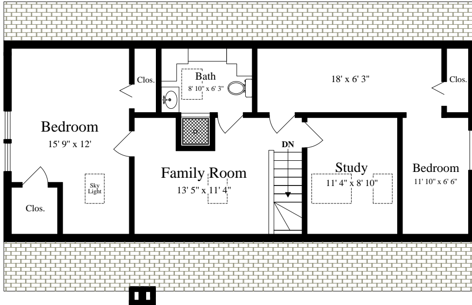
THIRD FLOOR (ceiling = 7' 4")
