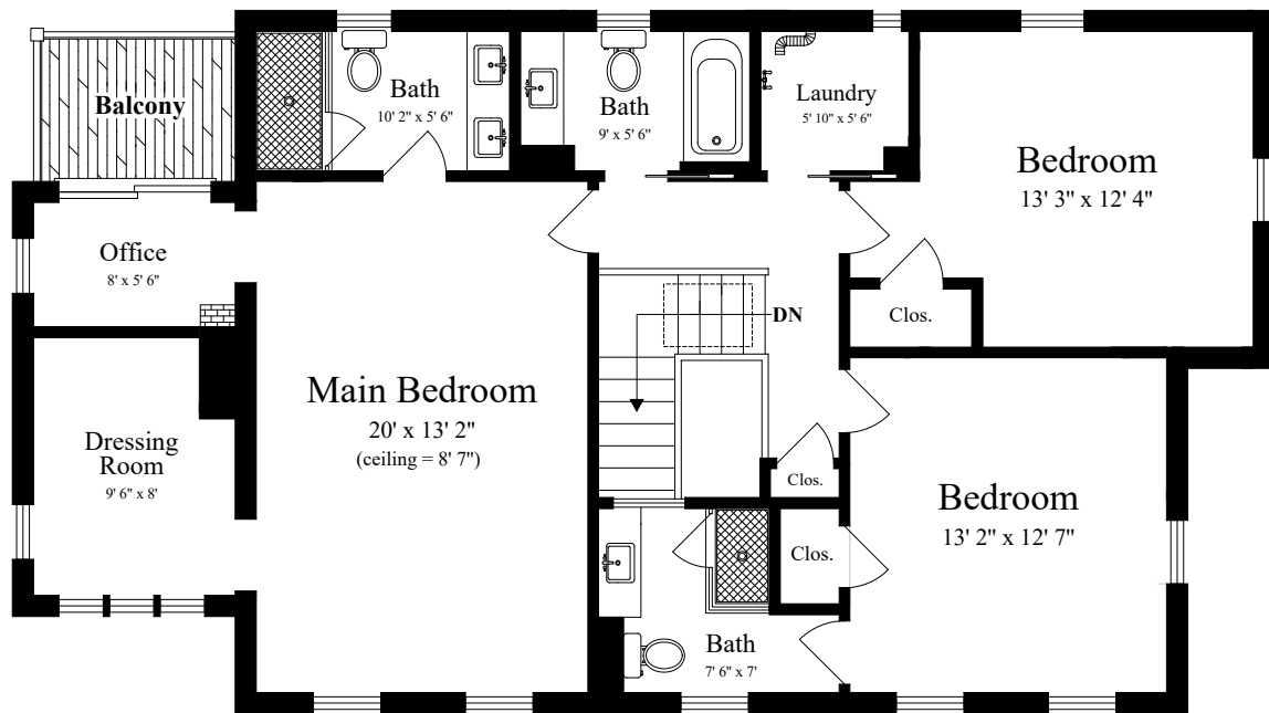
SECOND FLOOR (ceiling = 7' 7")
