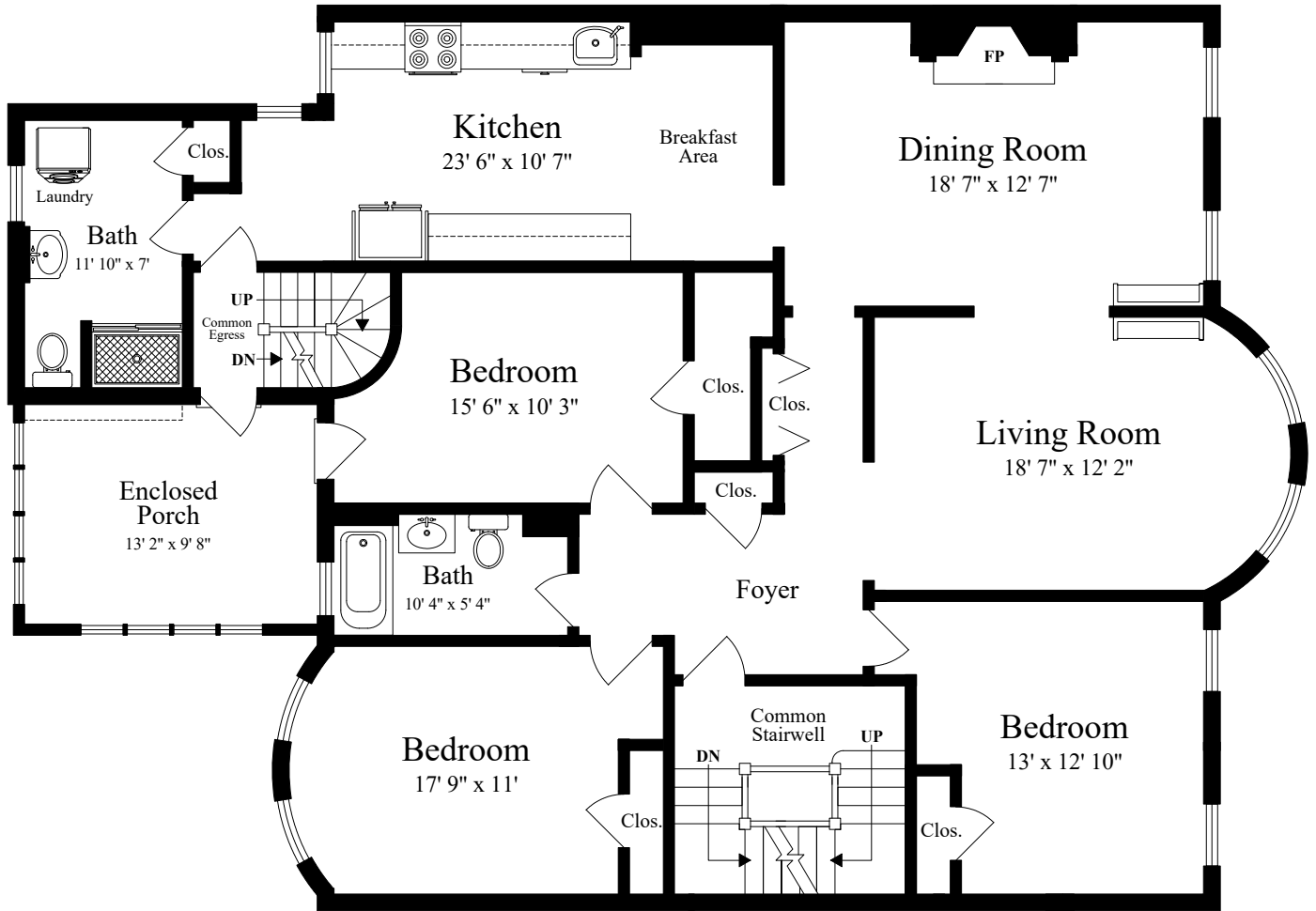
SECOND FLOOR
