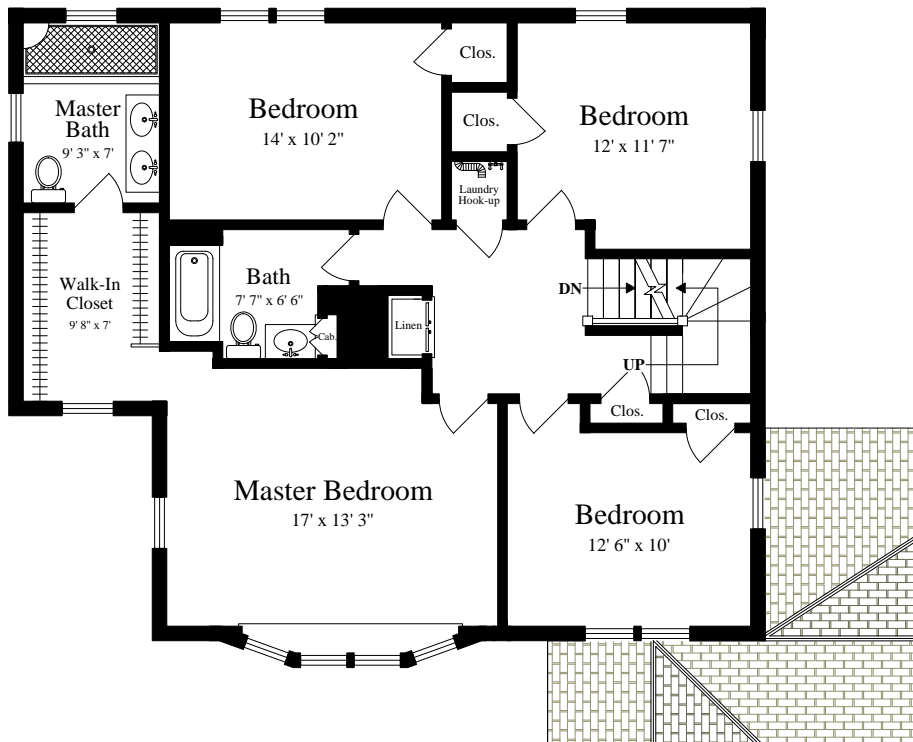
SECOND FLOOR (ceiling = 8')
