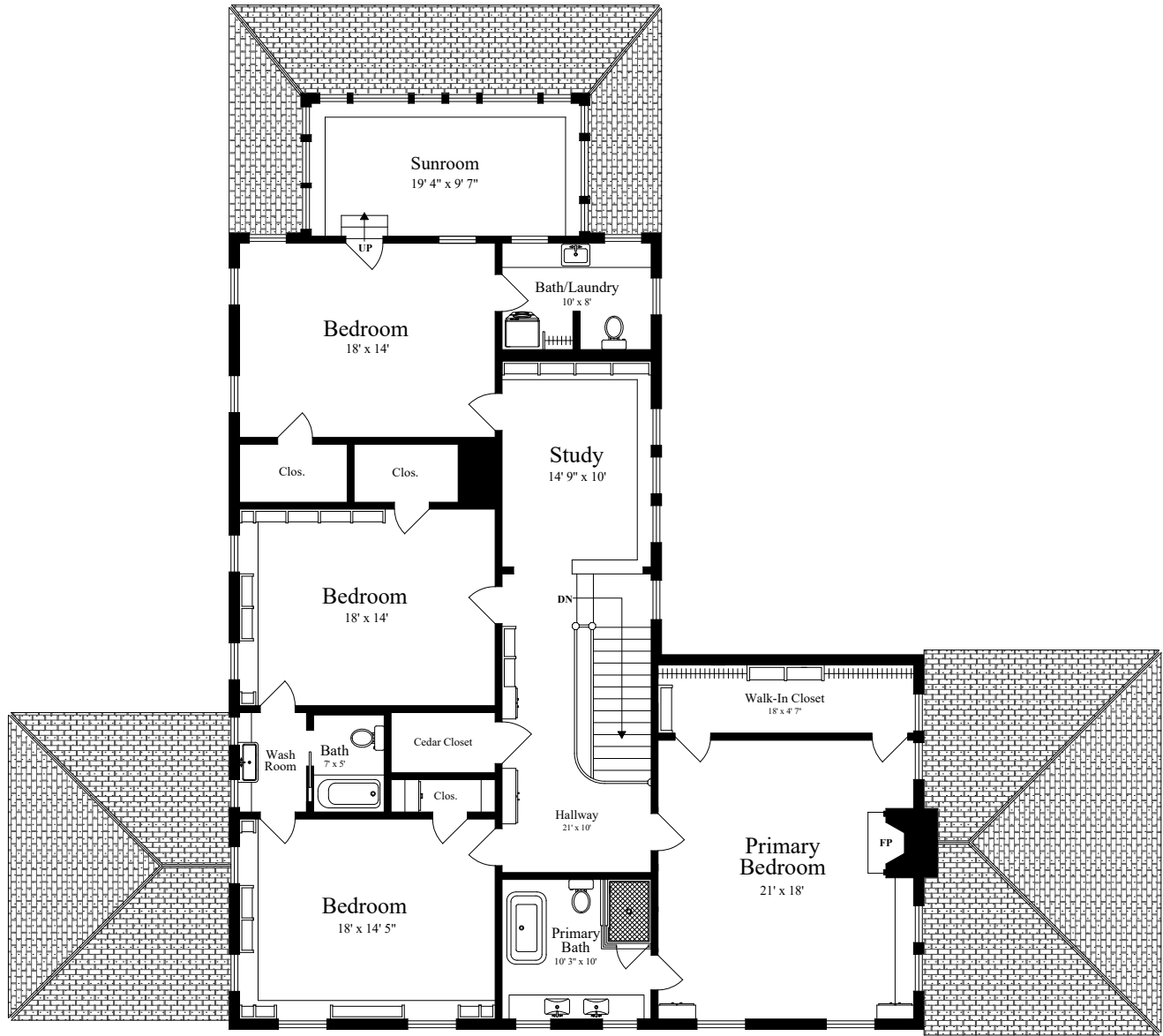
SECOND FLOOR (ceiling = 8' 6")
