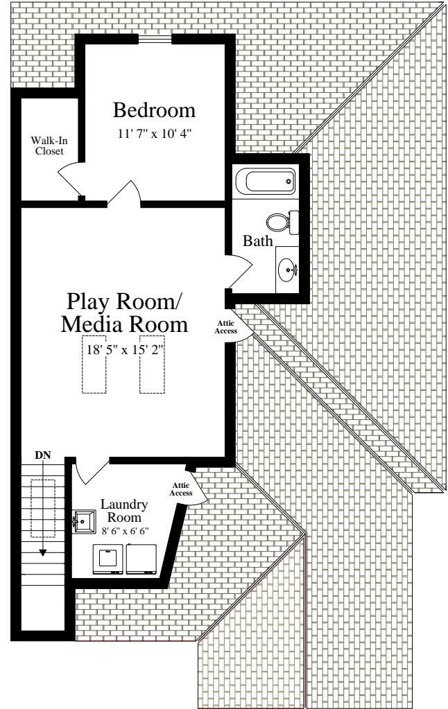
THIRD FLOOR (ceiling = 8')
