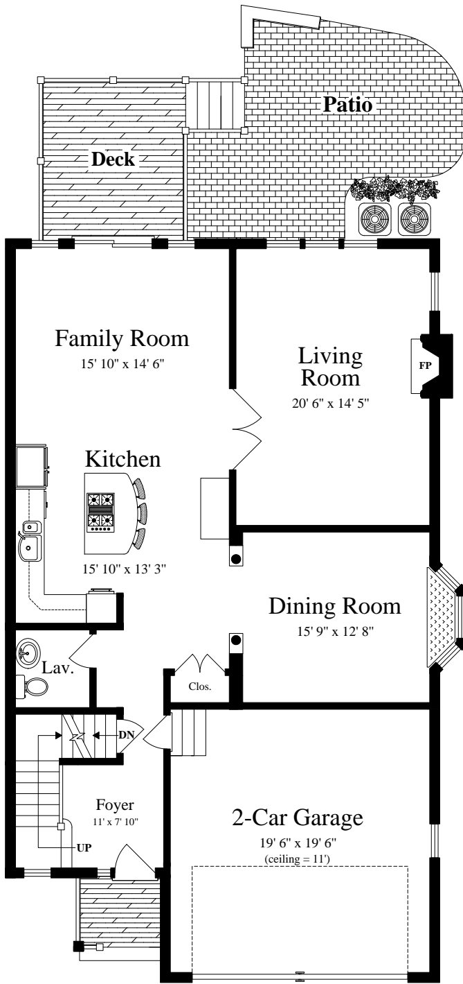
FIRST FLOOR (ceiling = 9')
