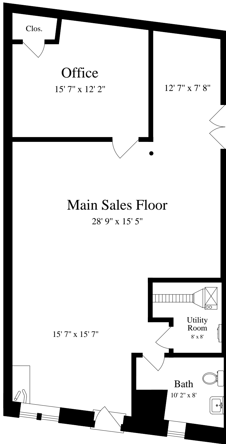
GROUND FLOOR (+/- 1050 sf ceiling = 7' 9")
