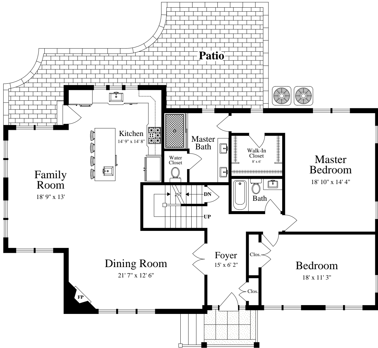
FIRST FLOOR (ceiling = 8' 10")
