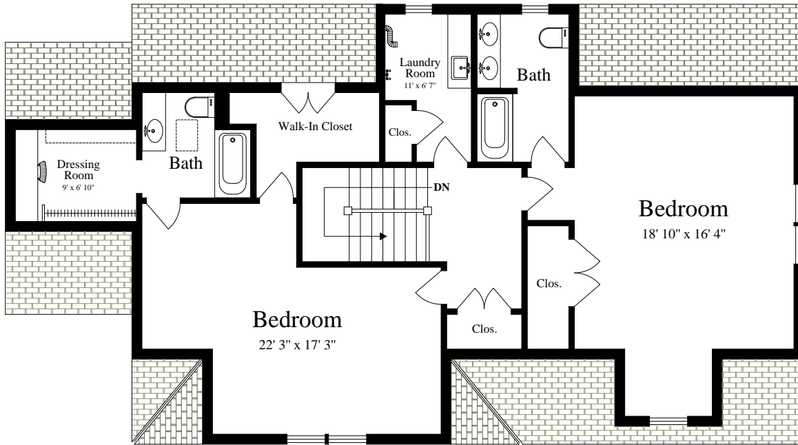
SECOND FLOOR (vaulted ceiling = 10')
