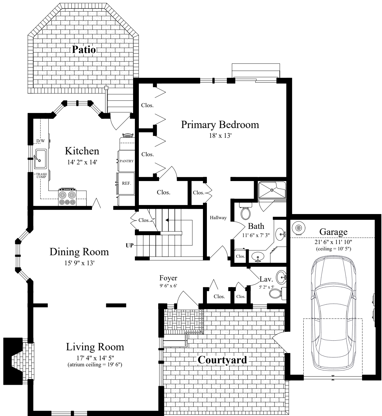
FIRST FLOOR (ceiling = 8')
