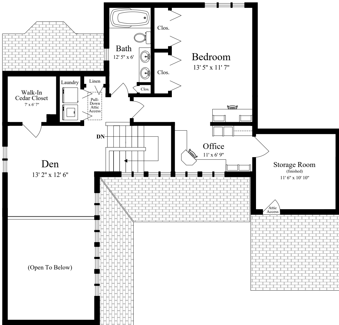
SECOND FLOOR (ceiling = 8')
