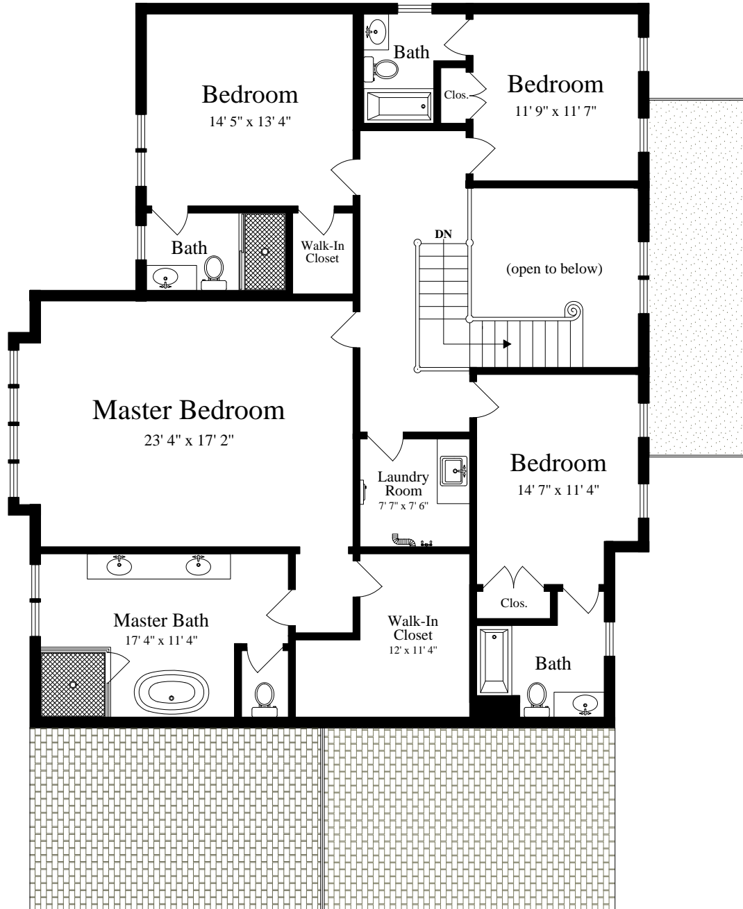
SECOND FLOOR (ceiling = 9')
