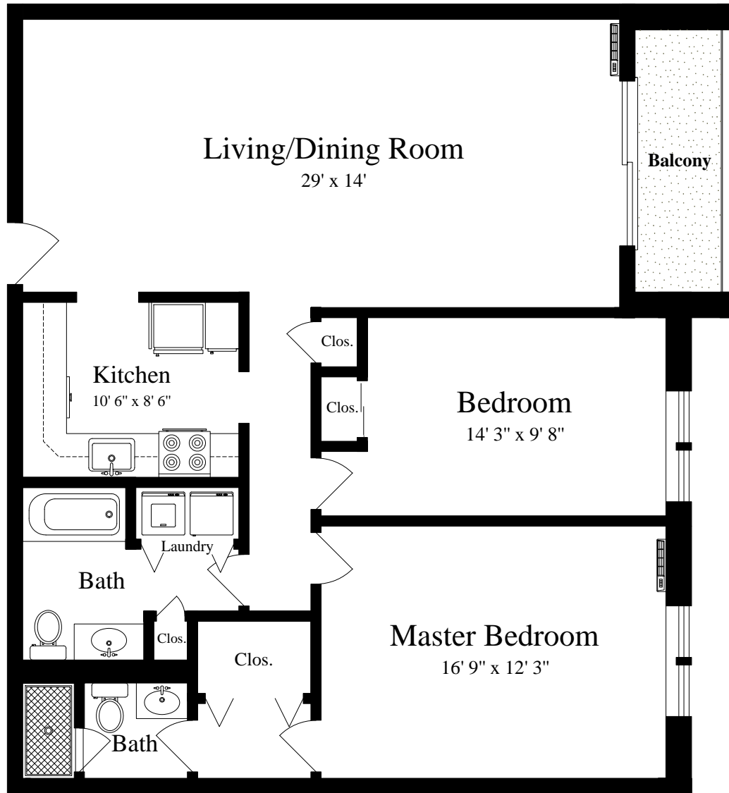
SECOND FLOOR (ceiling = 7' 3")
