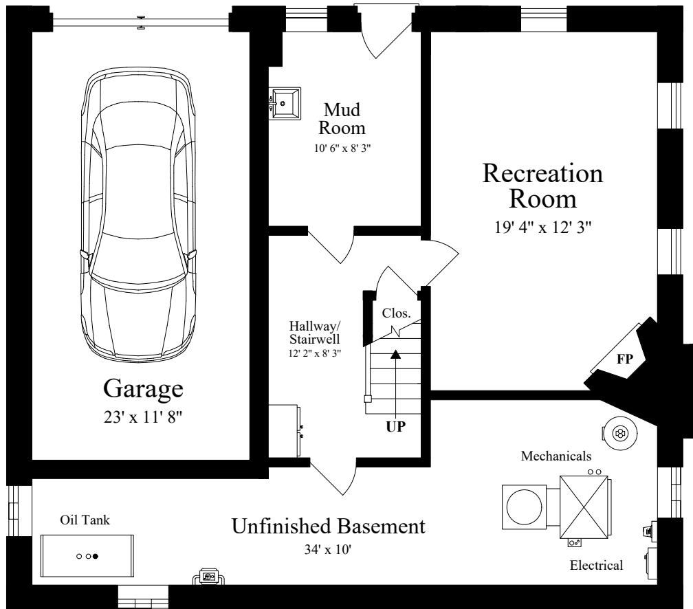
LOWER LEVEL (ceiling = 7' 9")
