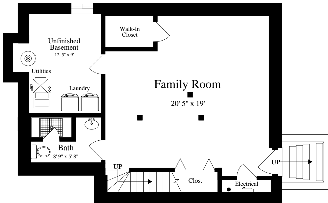
LOWER LEVEL (ceiling = 7' 3")
