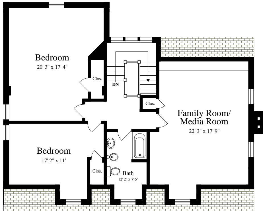
THIRD FLOOR (ceiling = 7' 2")
