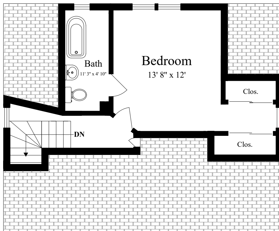
THIRD FLOOR (ceiling = 6' 4")
