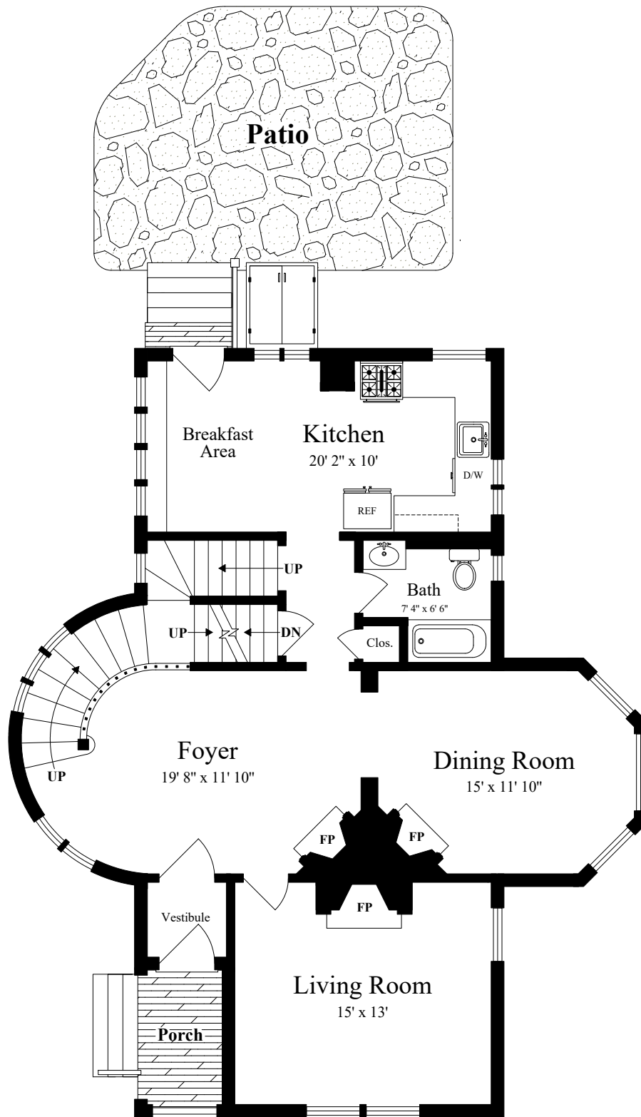
FIRST FLOOR (ceiling = 10')
