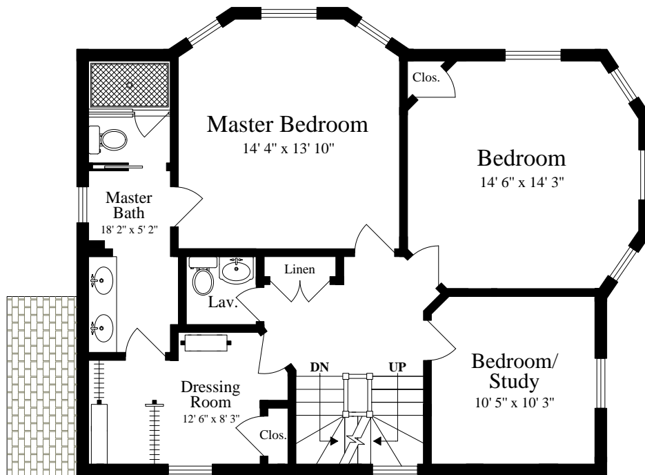
SECOND FLOOR (ceiling = 9')
