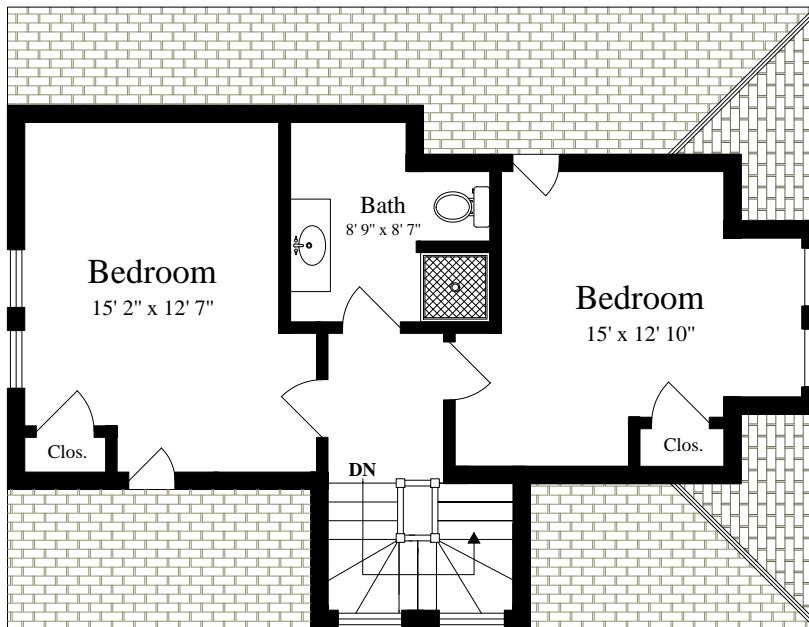
THIRD FLOOR (ceiling = 8' 7")
