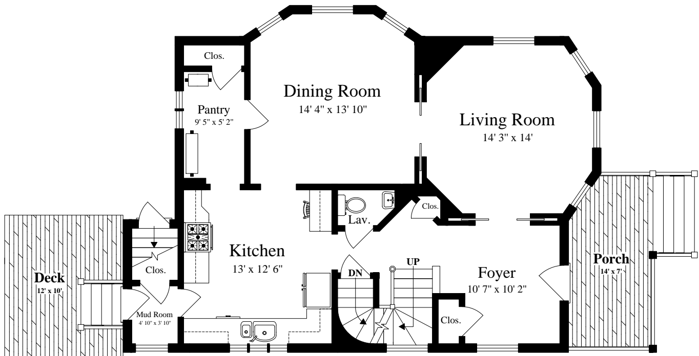
FIRST FLOOR (ceiling = 9')
