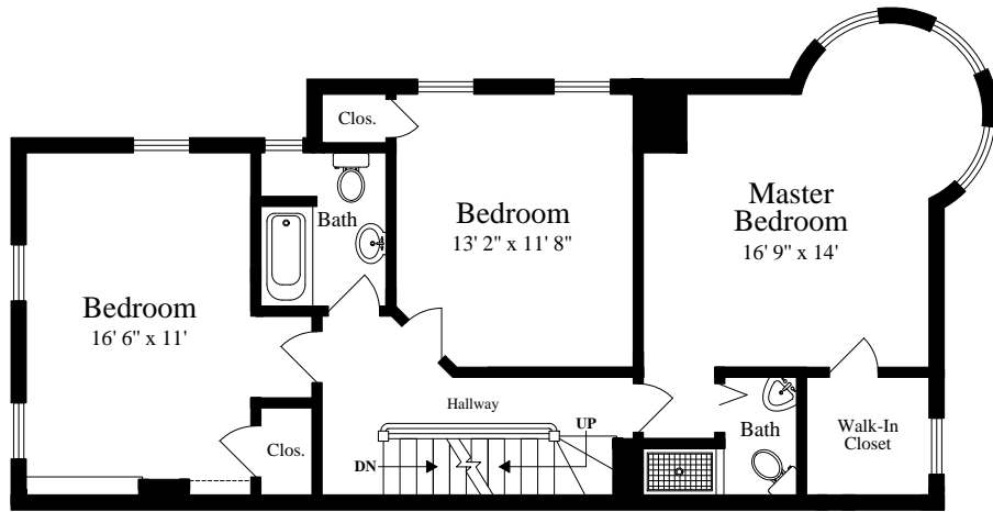
SECOND FLOOR
