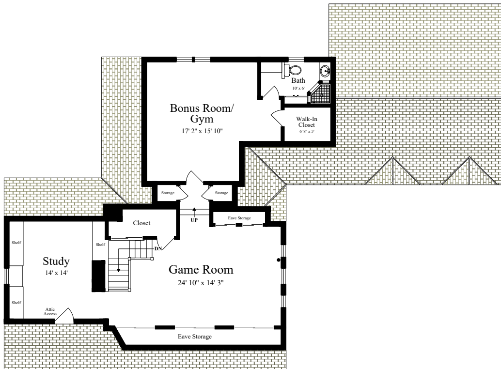
THIRD FLOOR (ceiling = 7' 9")
