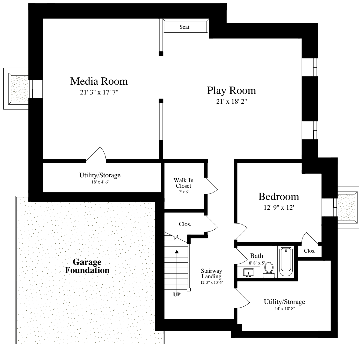
LOWER LEVEL (ceiling = 9')
