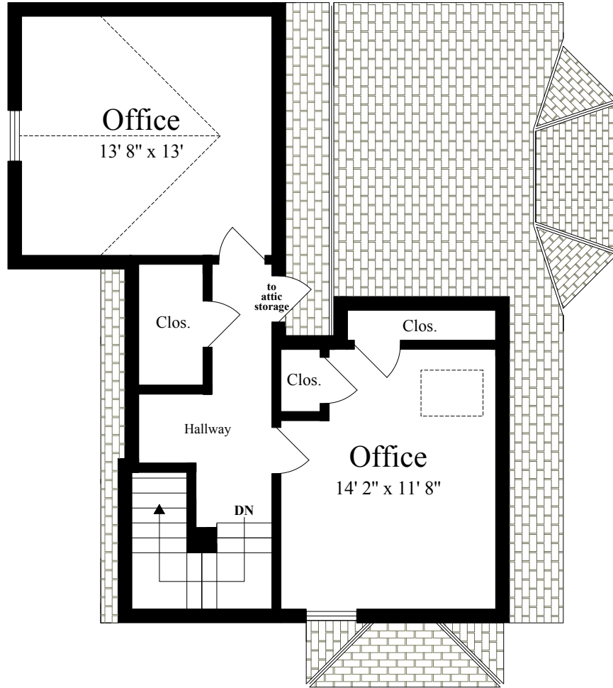
THIRD FLOOR (ceiling = 6' 10")
