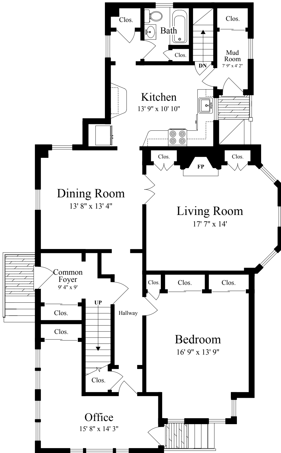
FIRST FLOOR (ceiling = 9')
