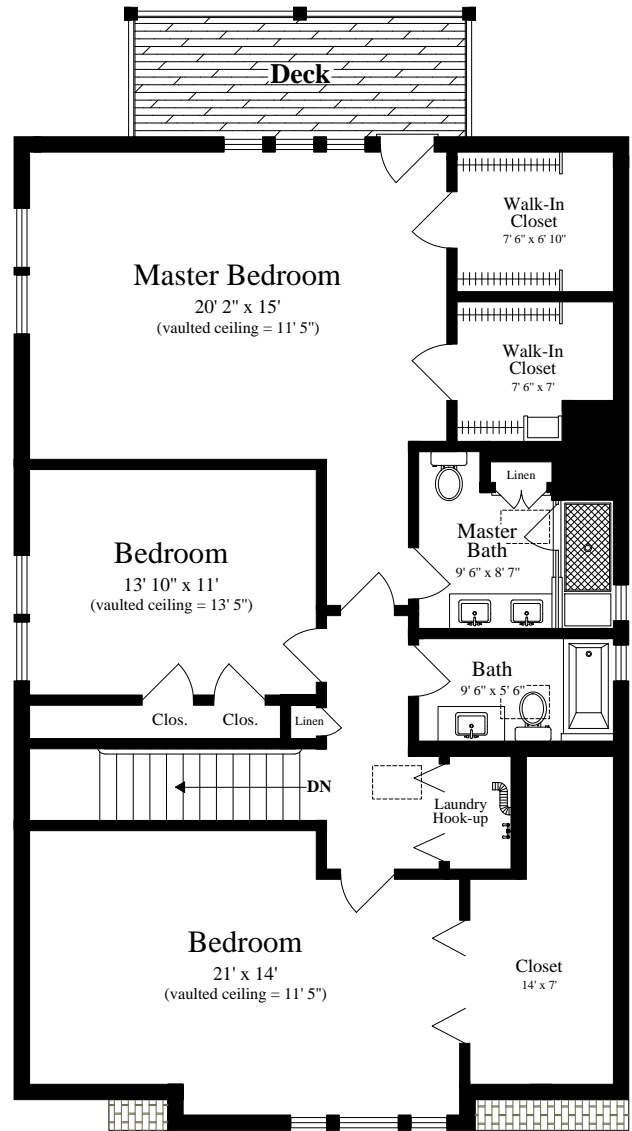
THIRD FLOOR (ceiling = 7' 10")
