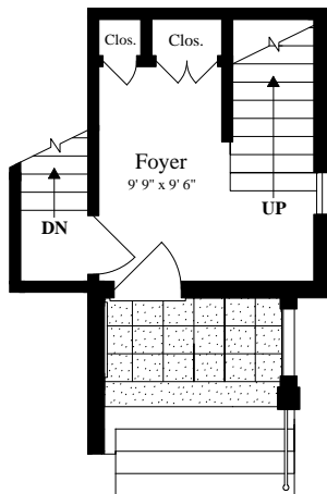
FIRST FLOOR (ceiling = 9')
