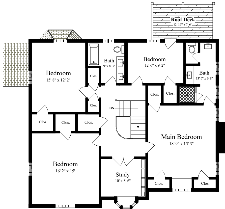
SECOND FLOOR (ceiling = 8' 2")
