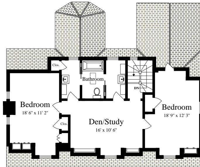
THIRD FLOOR (ceiling = 8' 2")
