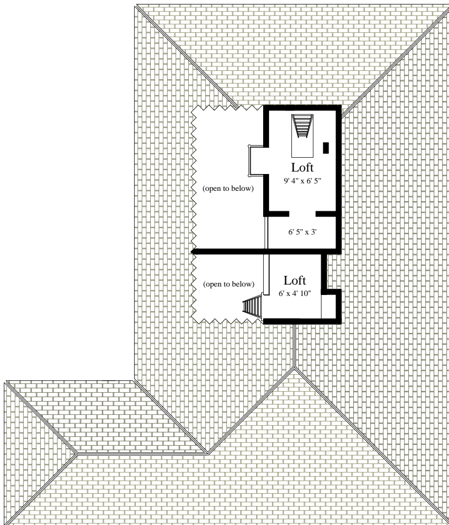
THIRD FLOOR (ceiling = 6')
