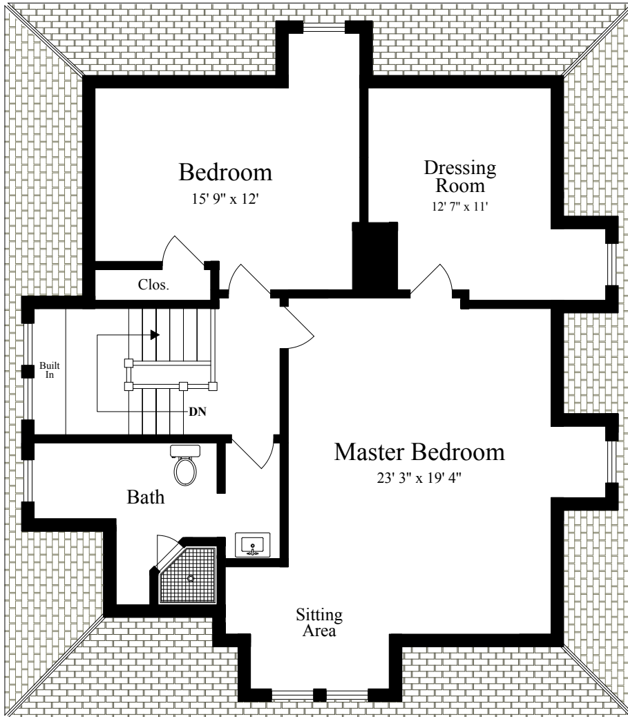
THIRD FLOOR
