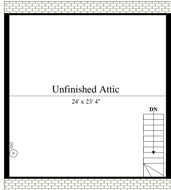
THIRD FLOOR (ceiling = 9' at center beam)
