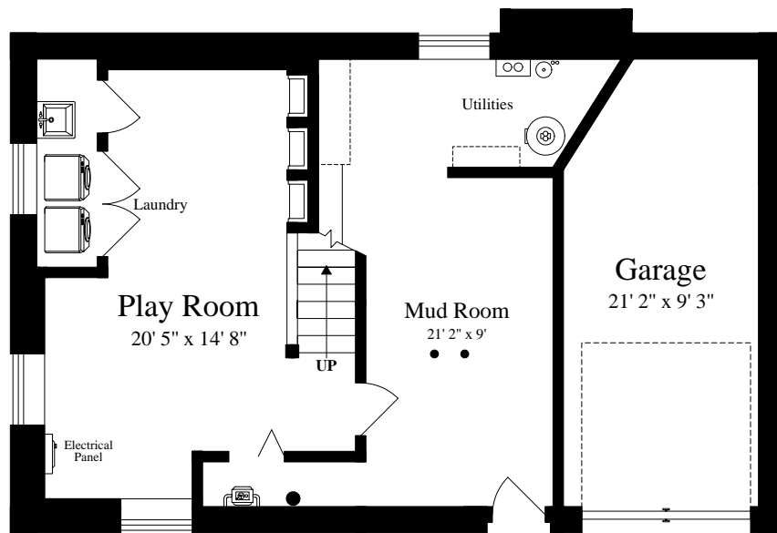
LOWER LEVEL (ceiling = 7' 2")
