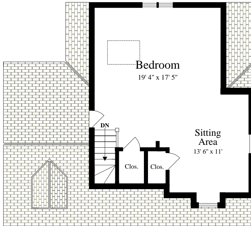
THIRD FLOOR (ceiling = 8' 3")
