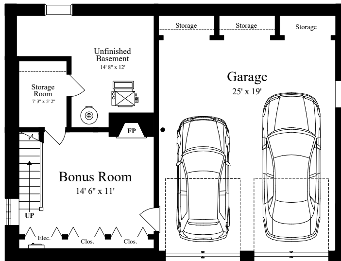
LOWER LEVEL (ceiling = 7' 3")
