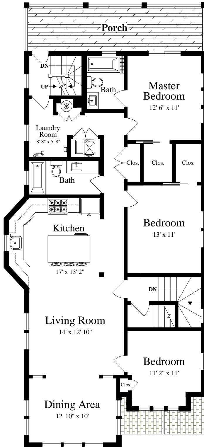
SECOND FLOOR (ceiling = 8' 9")
