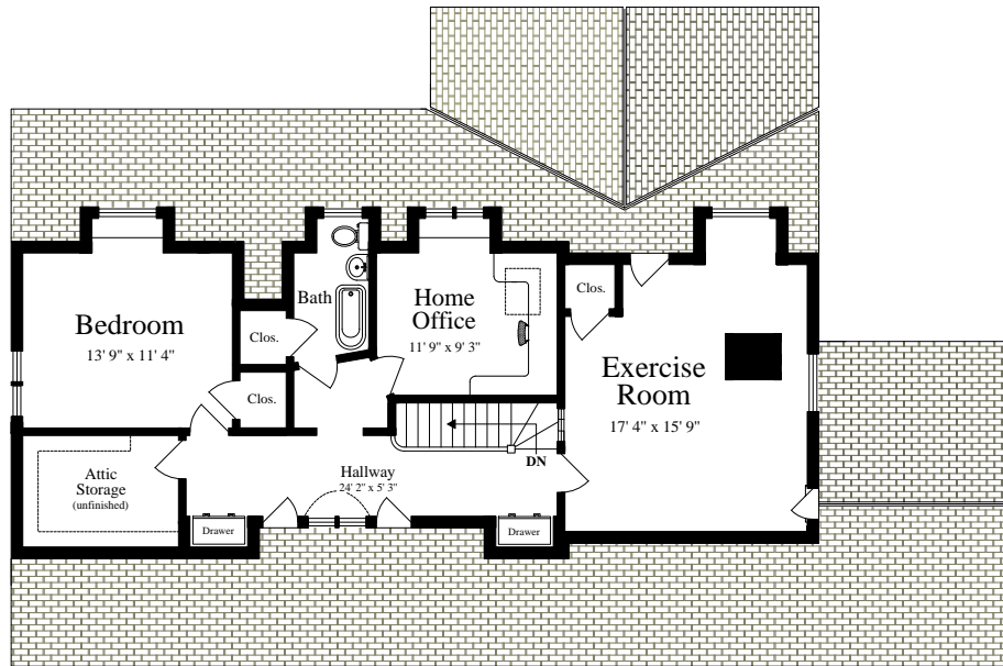
THIRD FLOOR (ceiling = 7' 6")
