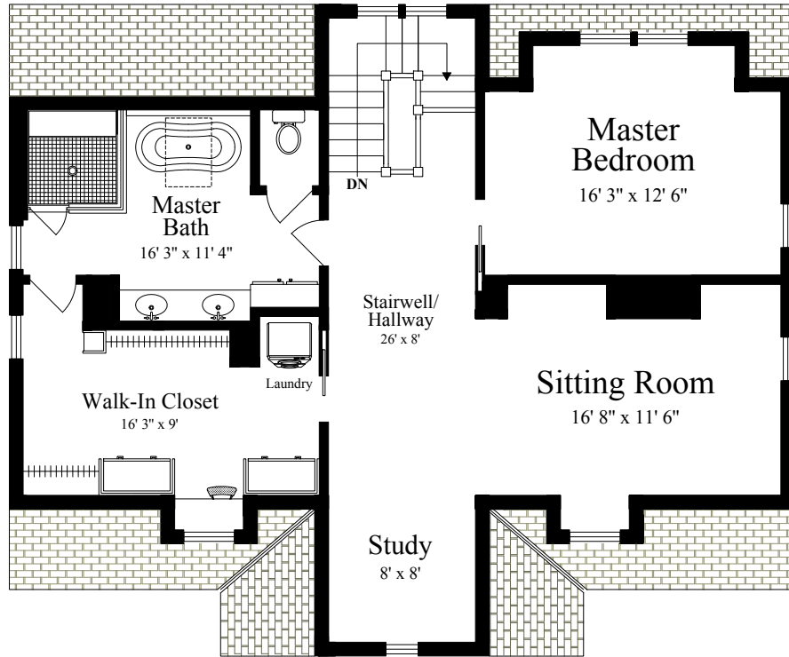
THIRD FLOOR (vaulted ceiling = 9' 7")
