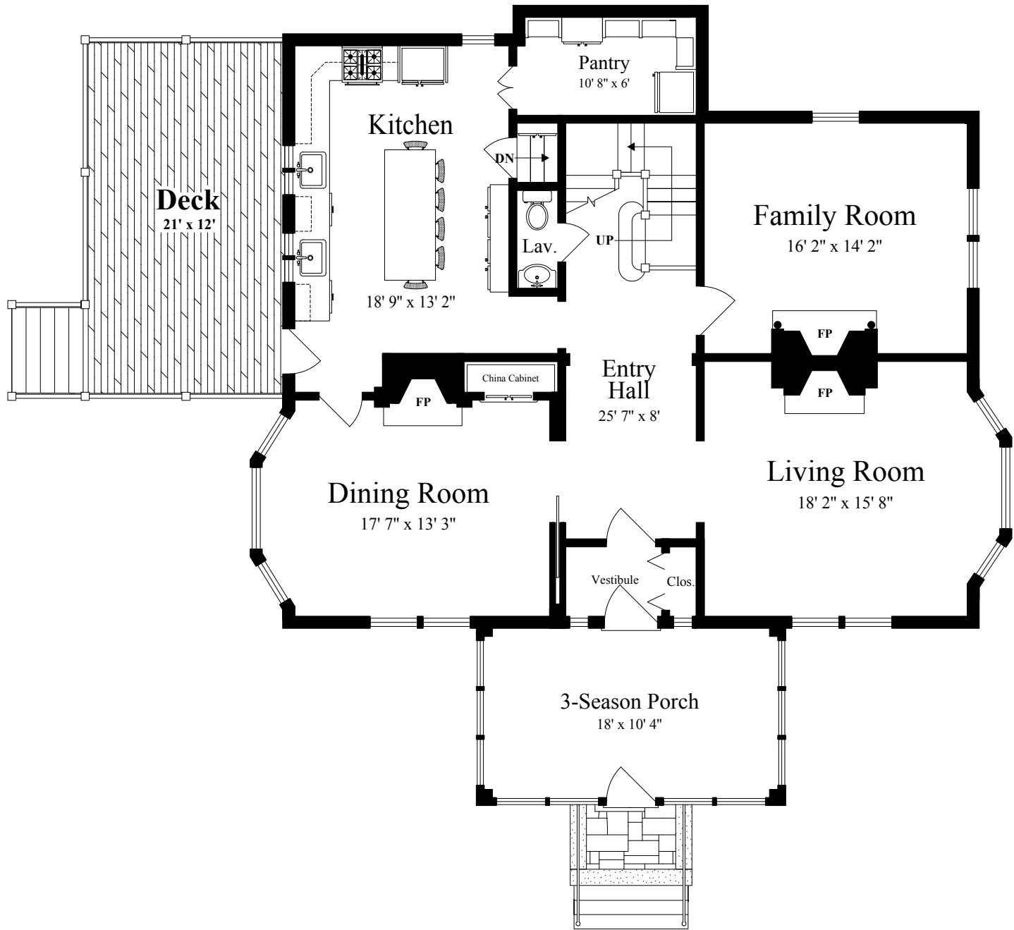
FIRST FLOOR (ceiling = 9')
