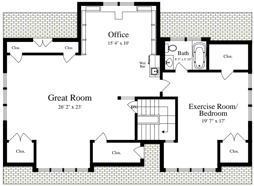
THIRD FLOOR (vaulted ceiling = 10' 10")
