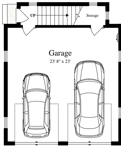
FIRST FLOOR (ceiling = 9' 9")
