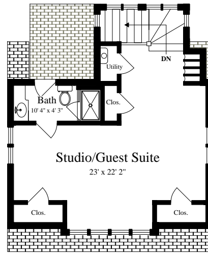
SECOND FLOOR (vaulted ceiling = 9')
