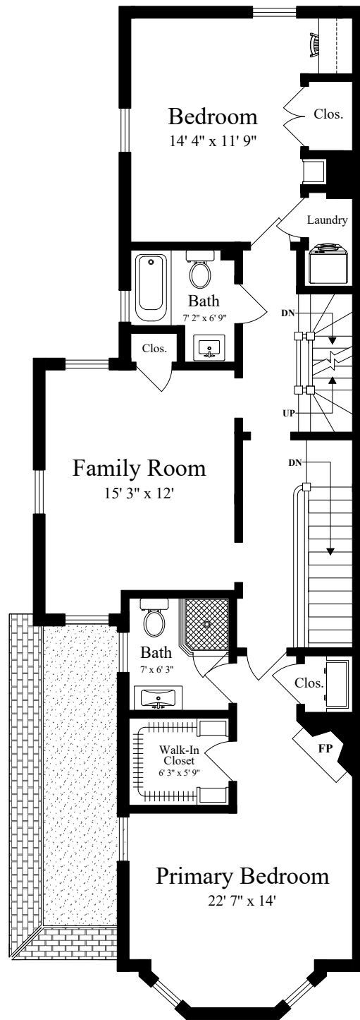
SECOND FLOOR (ceiling = 8')
