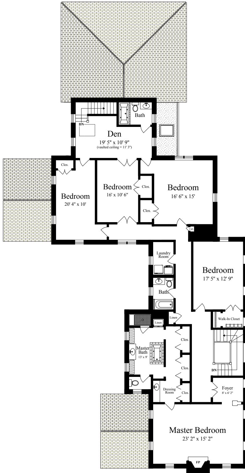
SECOND FLOOR (ceiling = 7' 7")
