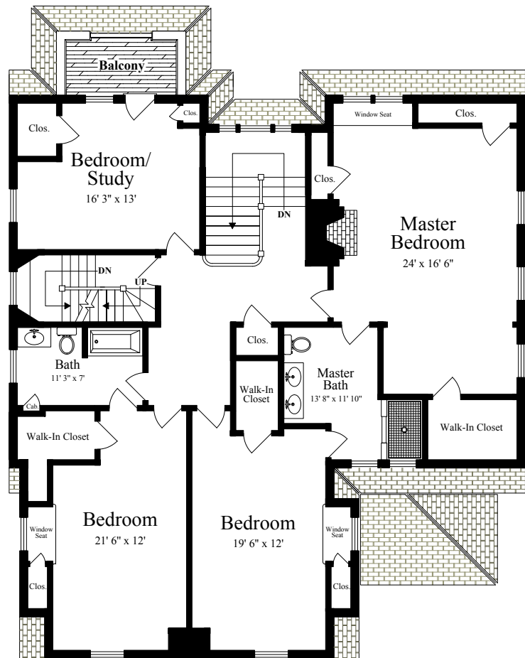
SECOND FLOOR (ceiling = 8' 6')
