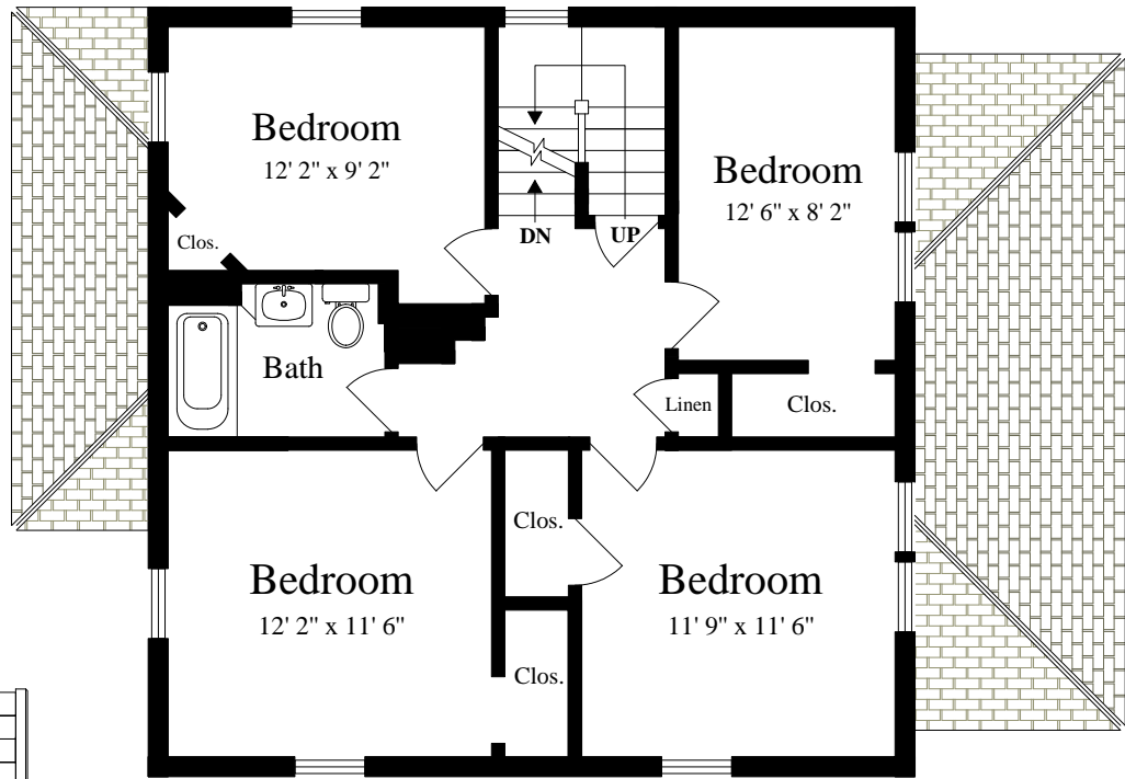
SECOND FLOOR (ceiling = 7' 9")
