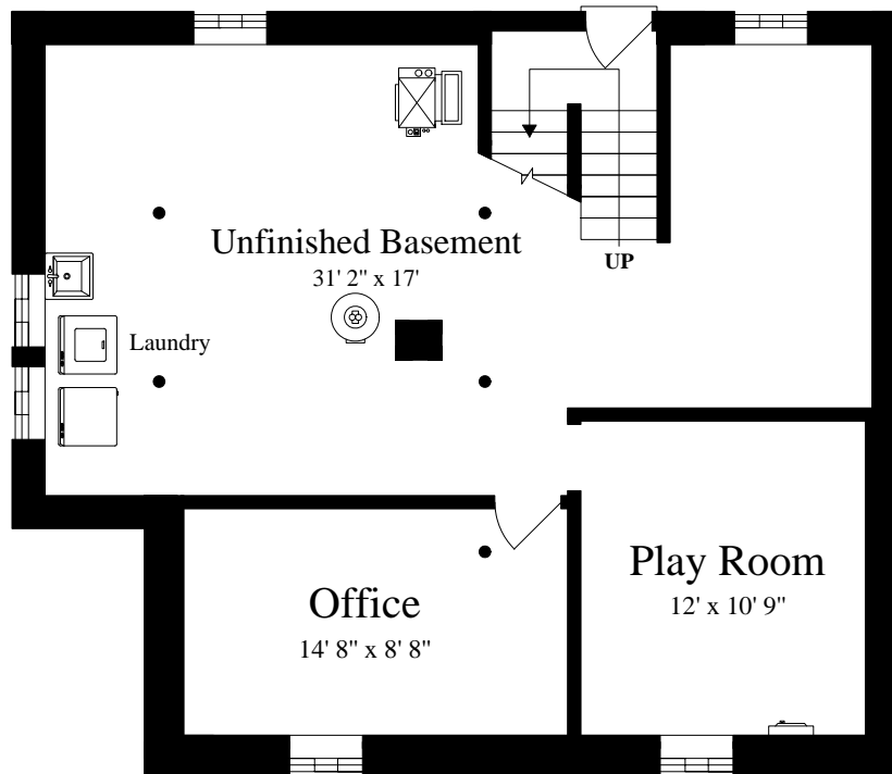
LOWER LEVEL (ceiling = 7' 4")
