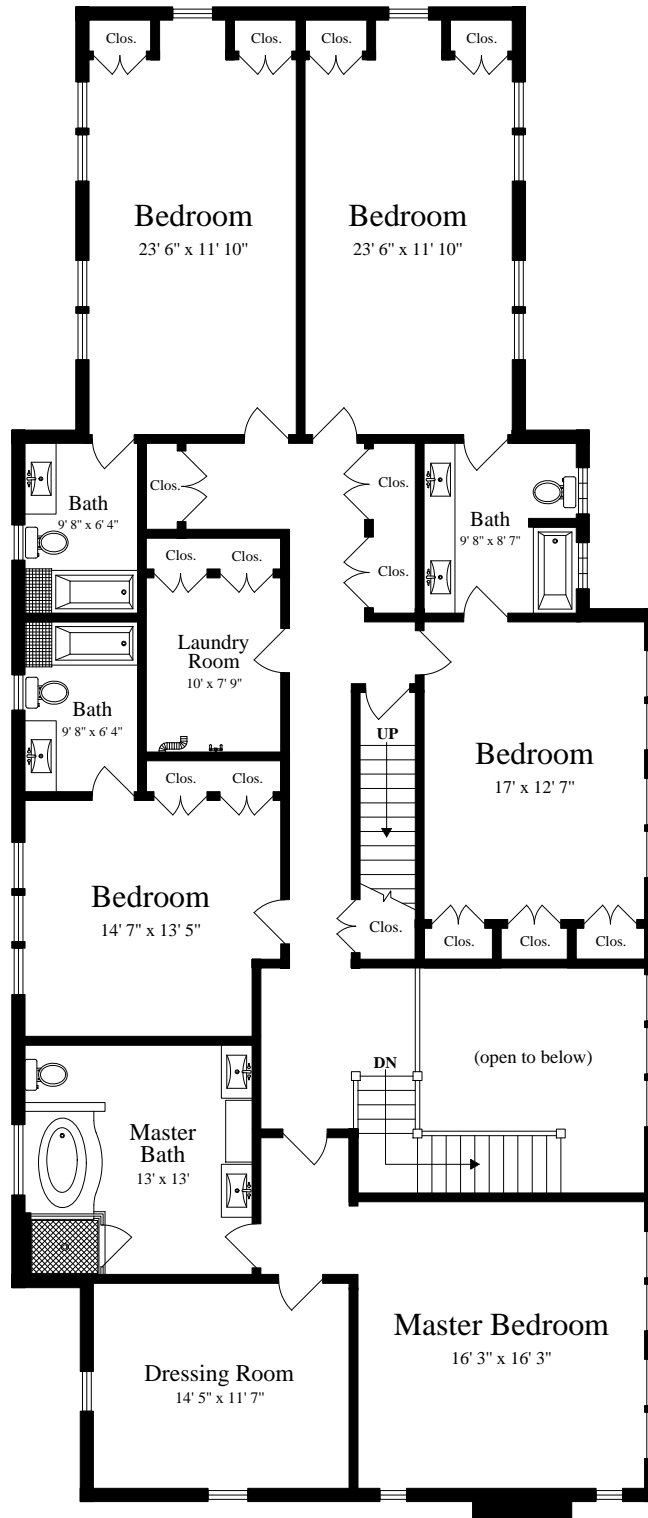
SECOND FLOOR (ceiling = 8' 9")
