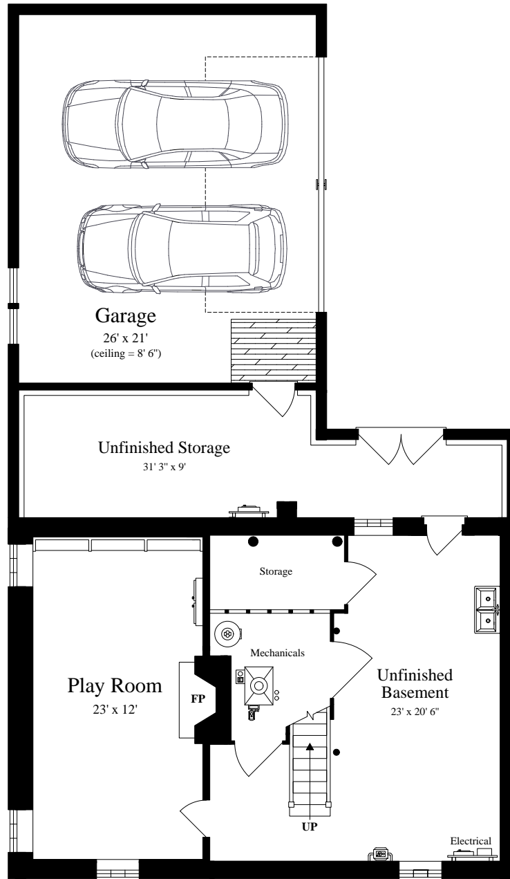
LOWER LEVEL (ceiling = 7' 3")
