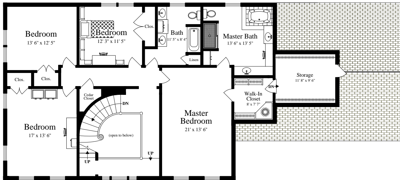
SECOND FLOOR (ceiling = 8' 2")
