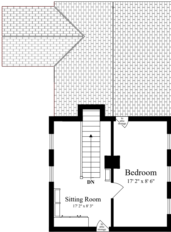
THIRD FLOOR (ceiling = 6' 6")
