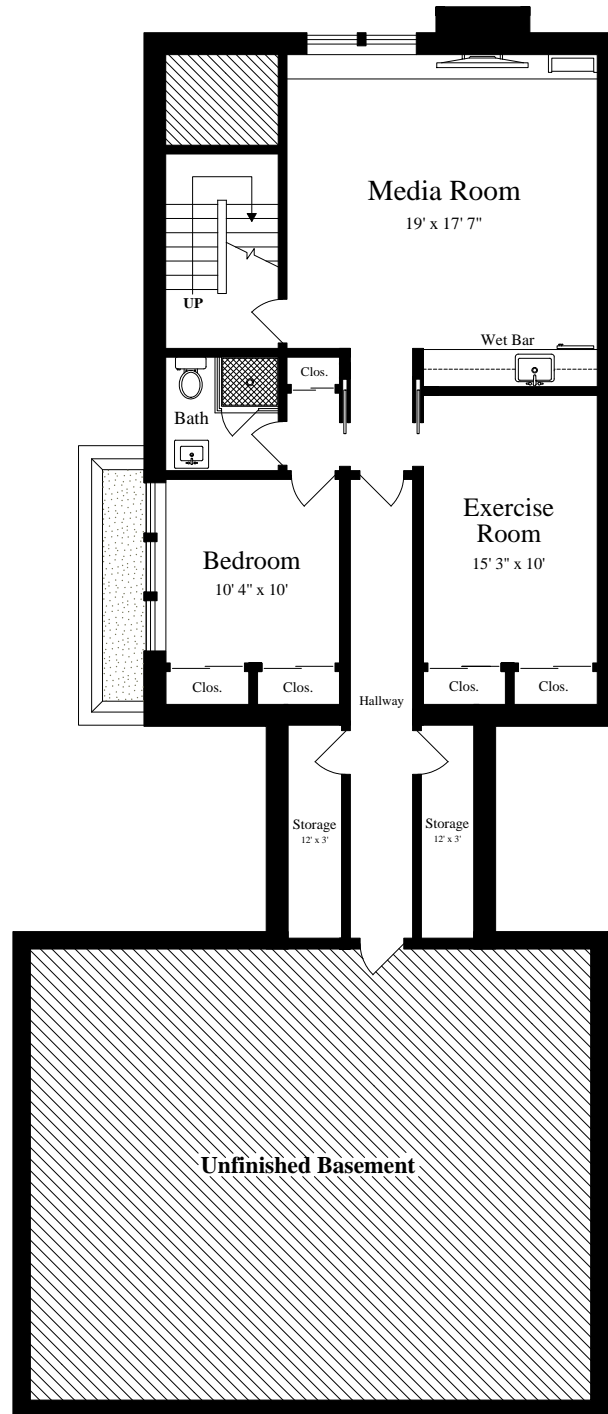
LOWER LEVEL (ceiling = 7' 10")
