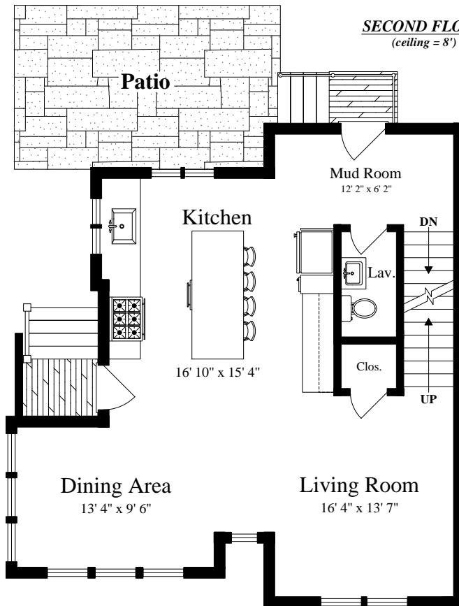
FIRST FLOOR (ceiling = 8')
