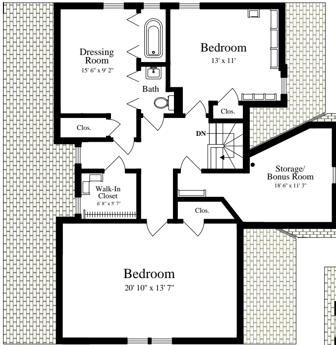
THIRD FLOOR (ceiling = 7' 9")
