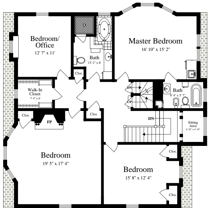
SECOND FLOOR (ceiling = 7' 10")
