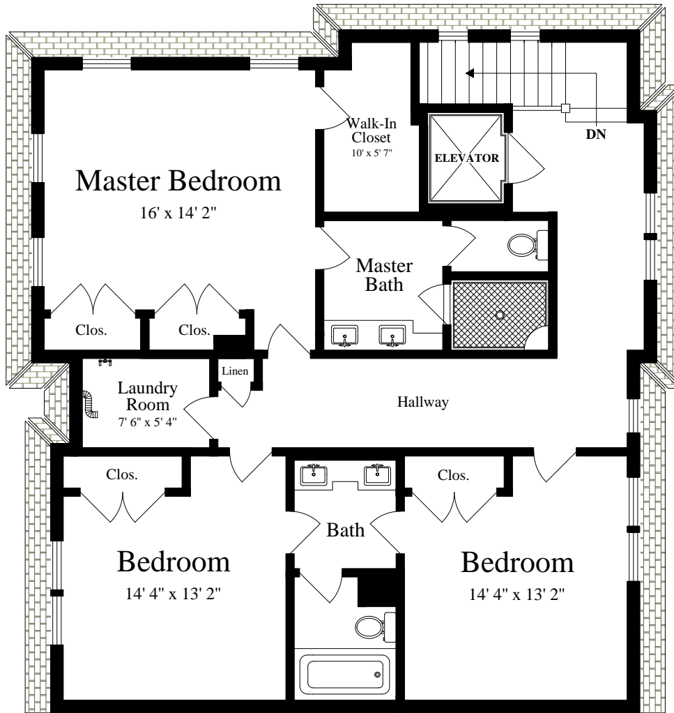
THIRD FLOOR (ceiling = 8' 4")
