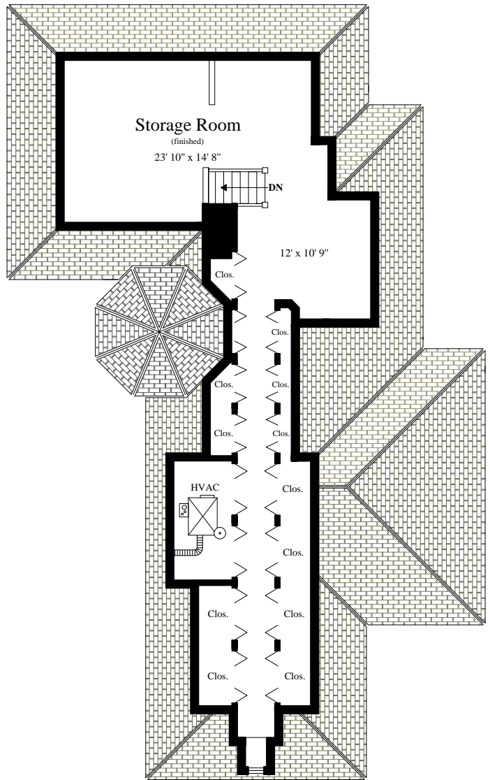
THIRD FLOOR (ceiling = 7' 4")
