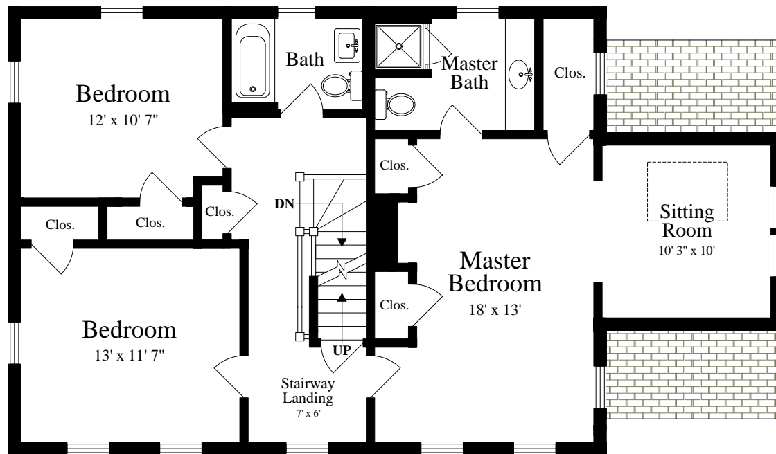
SECOND FLOOR (ceiling = 8')
