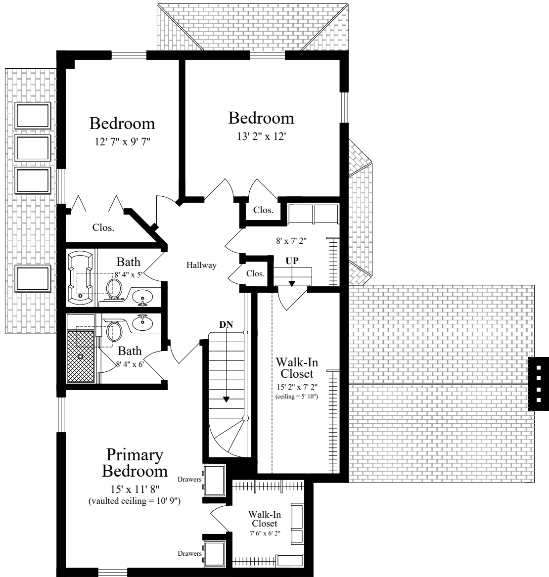
SECOND FLOOR (ceiling = 7' 6")
