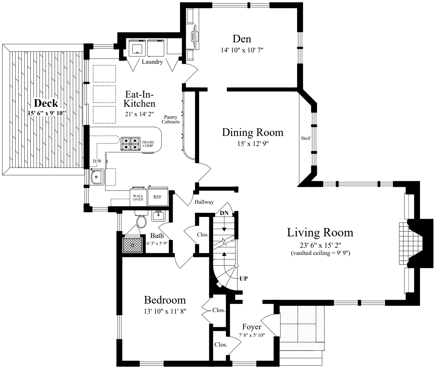
FIRST FLOOR (ceiling = 7' 10")
