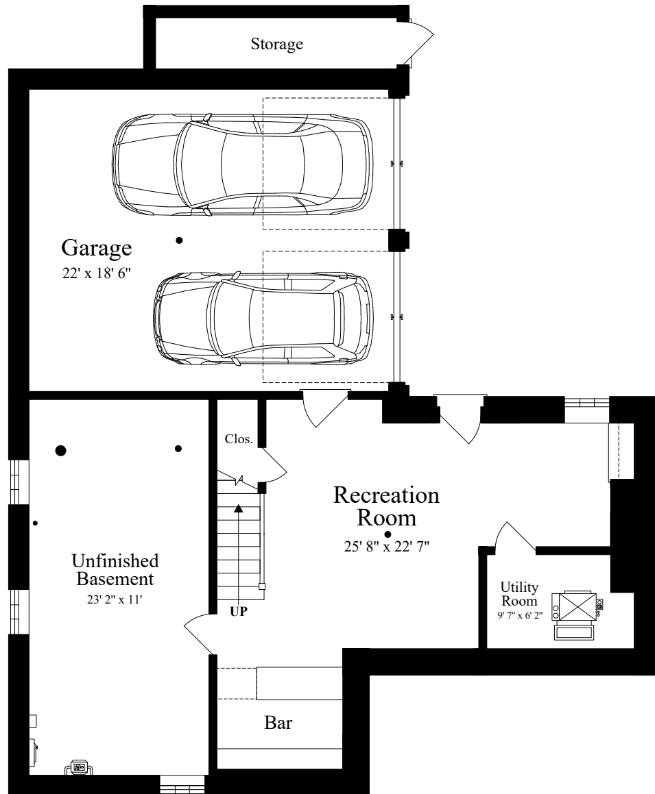
LOWER LEVEL (ceiling = 7' 3")
